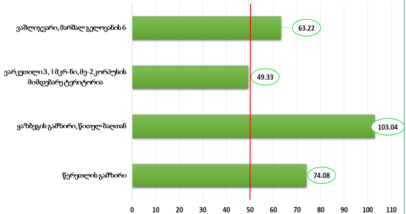
PM10, მკგ/მ3
