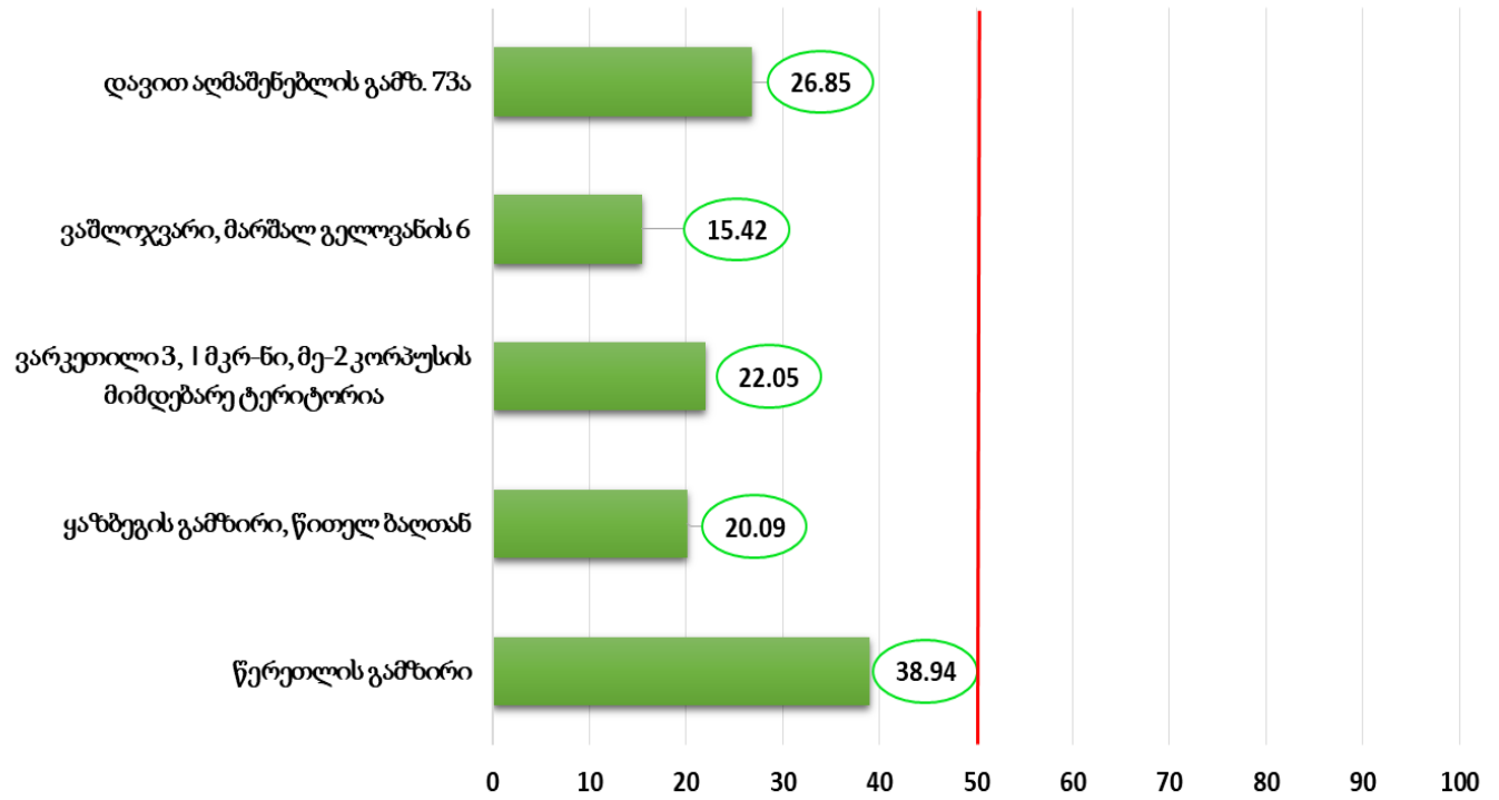
PM10, მკგ/მ3
