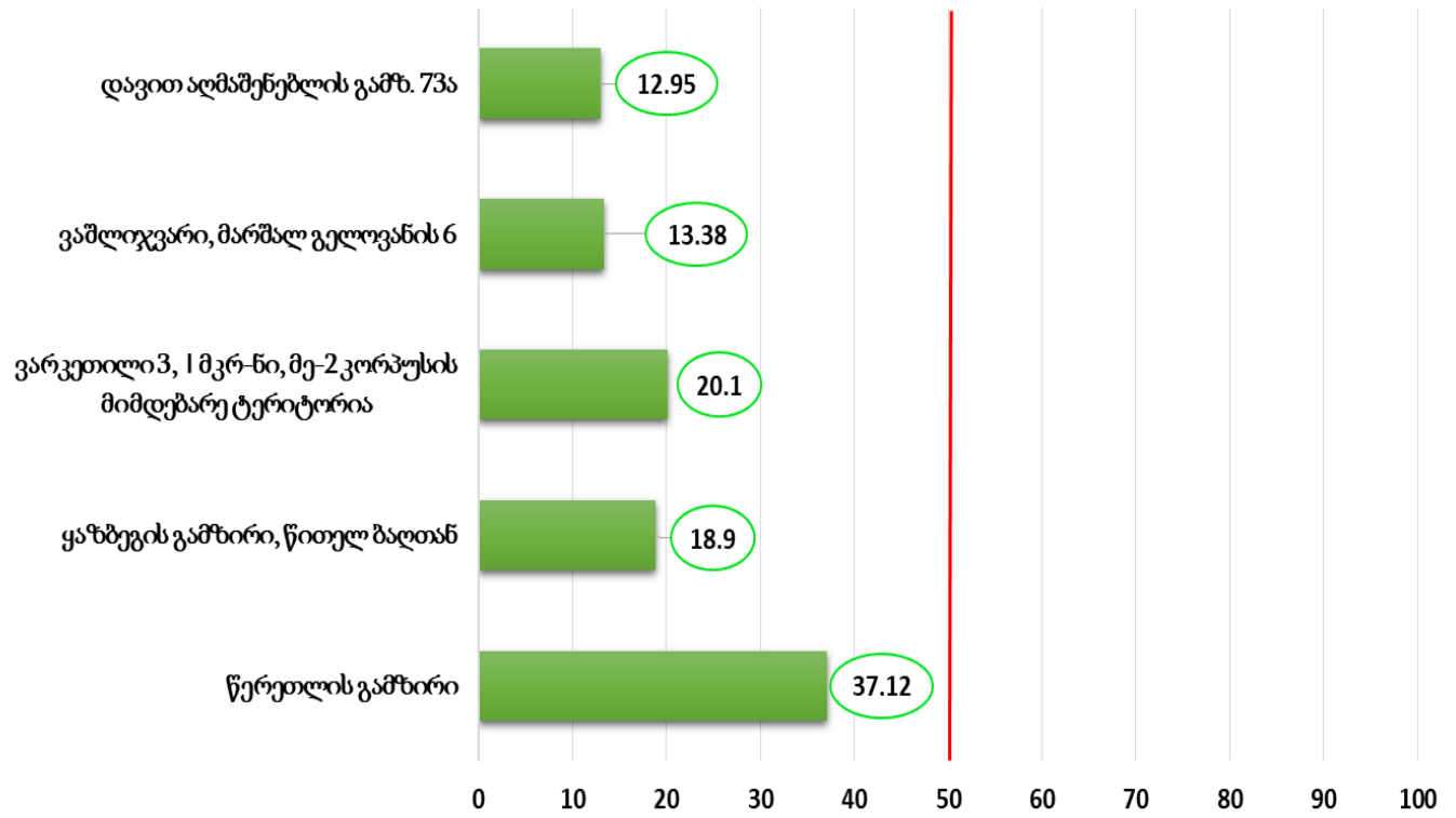
PM10, მკგ/მ3
