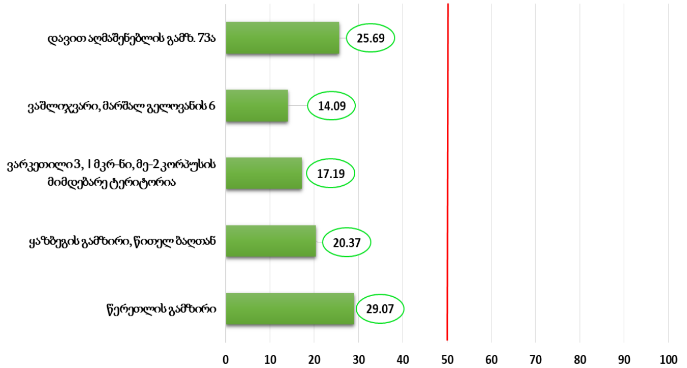
PM10, მკგ/მ3
