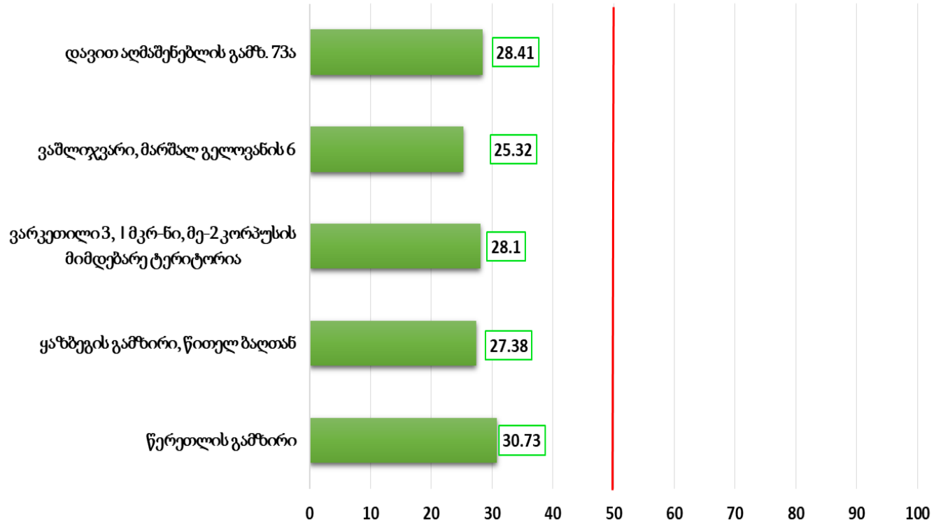
PM10, მკგ/მ3
