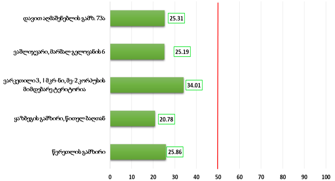
PM10, მკგ/მ3
