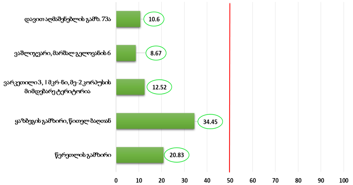
PM10, მკგ/მ3
