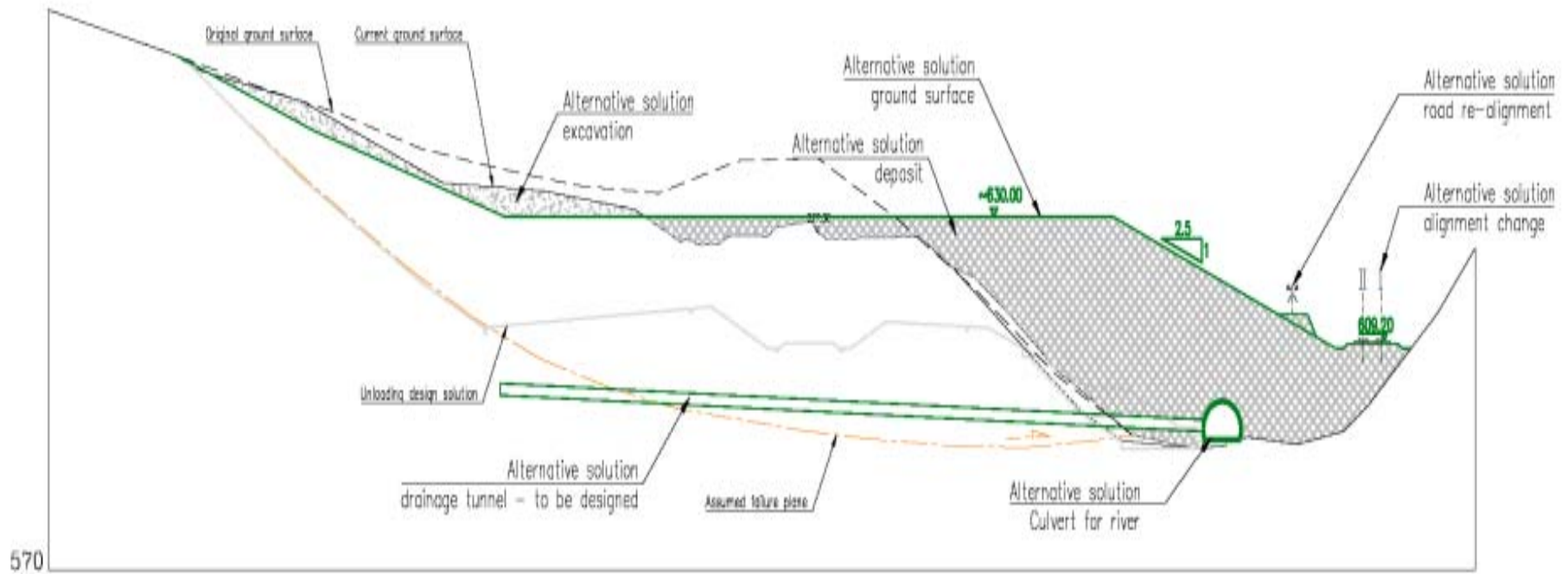
Cross Section of Landslide Km22+860
